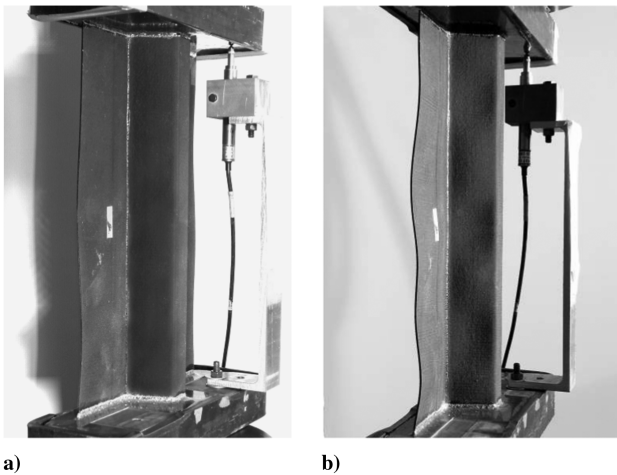
Fig. 4 Structural response of a single-stringer specimen with Teflon insert at two load levels: a) 15 kN; b) 35 kN.
