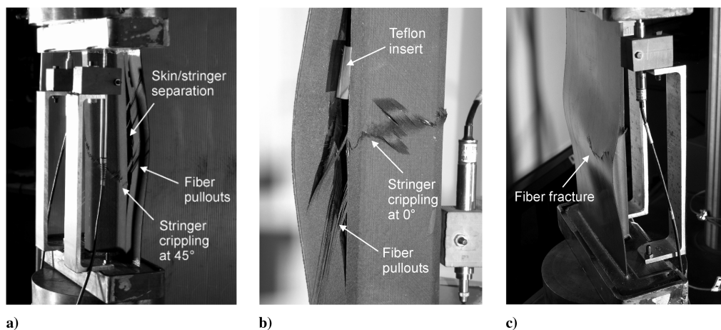
Fig. 5 Failure modes in different panels: a) initially pristine specimen; b) specimen with Teflon insert; c) specimen with Teflon insert (back side).
