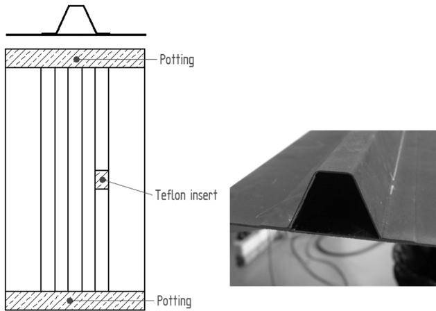
Fig. 3 Configuration of SSC specimen and closeup of hat stiffener.
