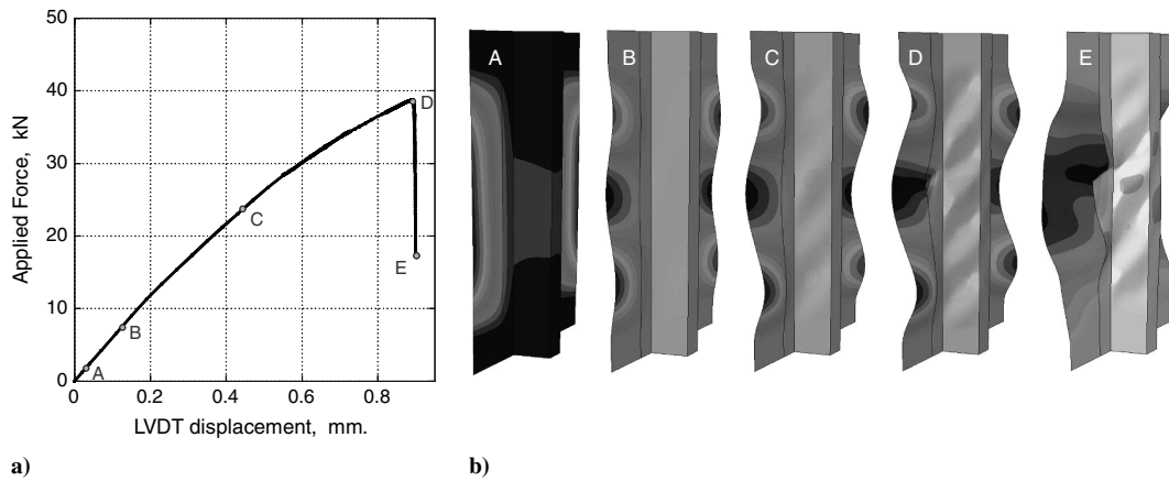
Fig. 7 Analysis of the nominally pristine specimen: a) load-displacement curve; b) out-of-plane response.
