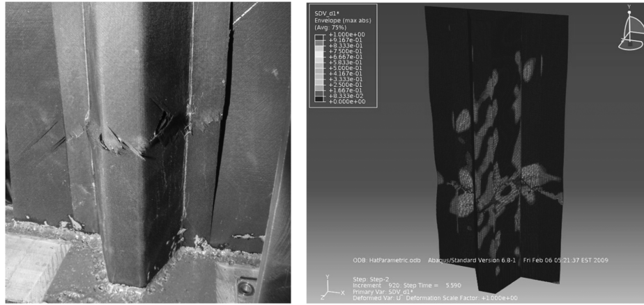
Fig. 12 Comparison between experimental and numerical collapse modes of a nominally pristine specimen.
