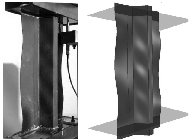
Fig. 11 Comparison between experimental and numerical postbuckling deformed shapes.
