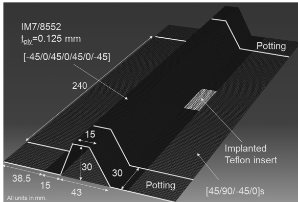
Fig. 6 Finite element model and dimensions of the SSC specimen.
