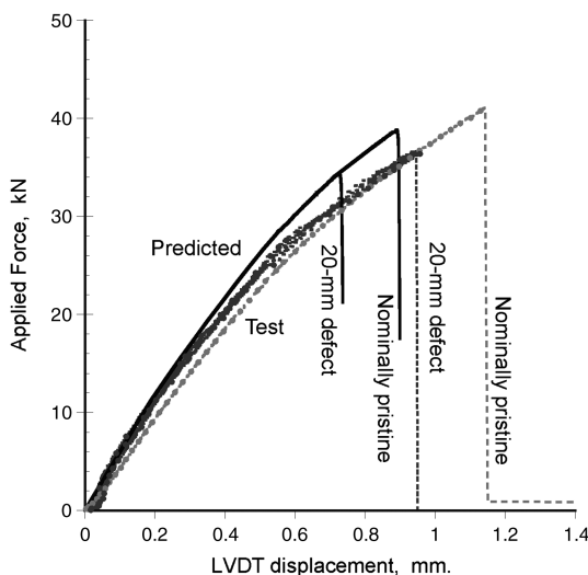
Fig. 10 Numerical and experimental force-displacement curves.
