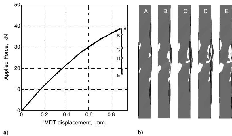
Fig. 9 Analysis of the nominally pristine specimen: a) load-displacement curve; b) skin/stringer separation (side view).
