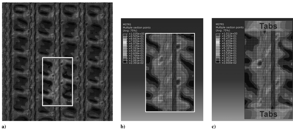
Fig. 2 Maximum stress contour plots for a) multistringer panel; b) subunit of the multistringer panel; c) SSC specimen.
