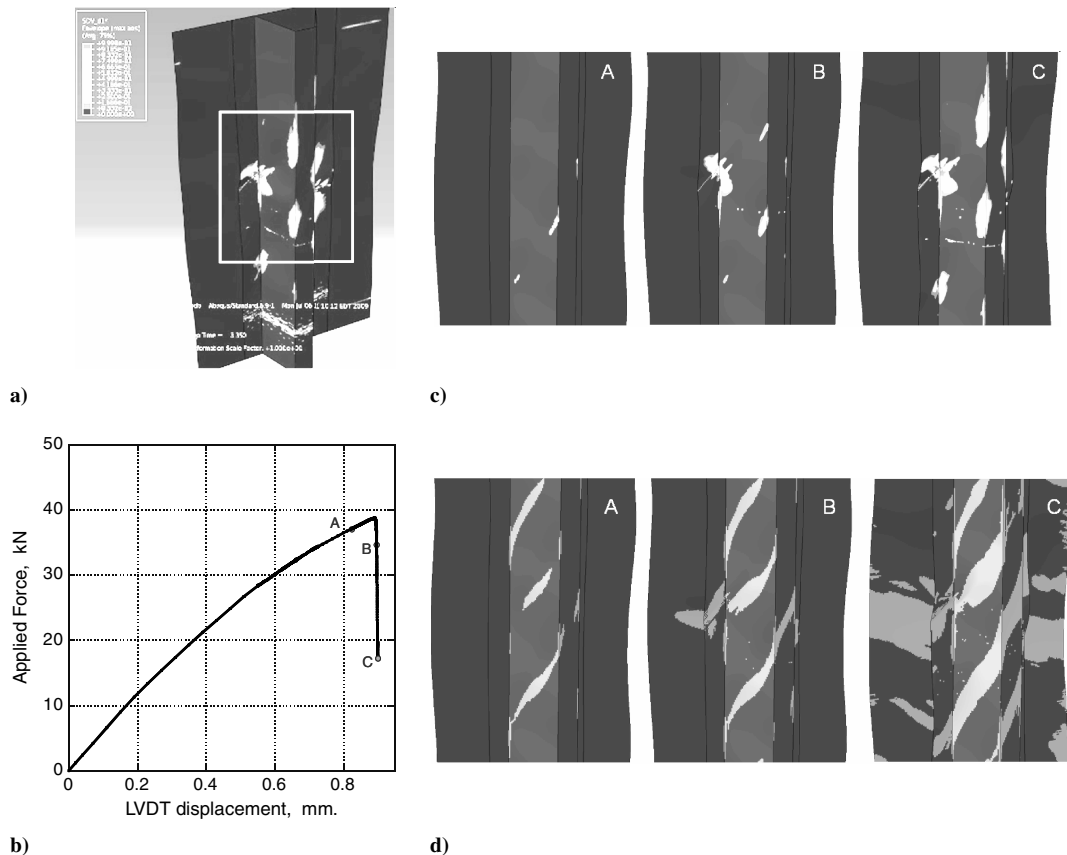
Fig. 8 Analysis of the nominally pristine specimen: a) damaged area on the specimen; b) load-displacement curve; c) fiber damage; d) matrix damage.
